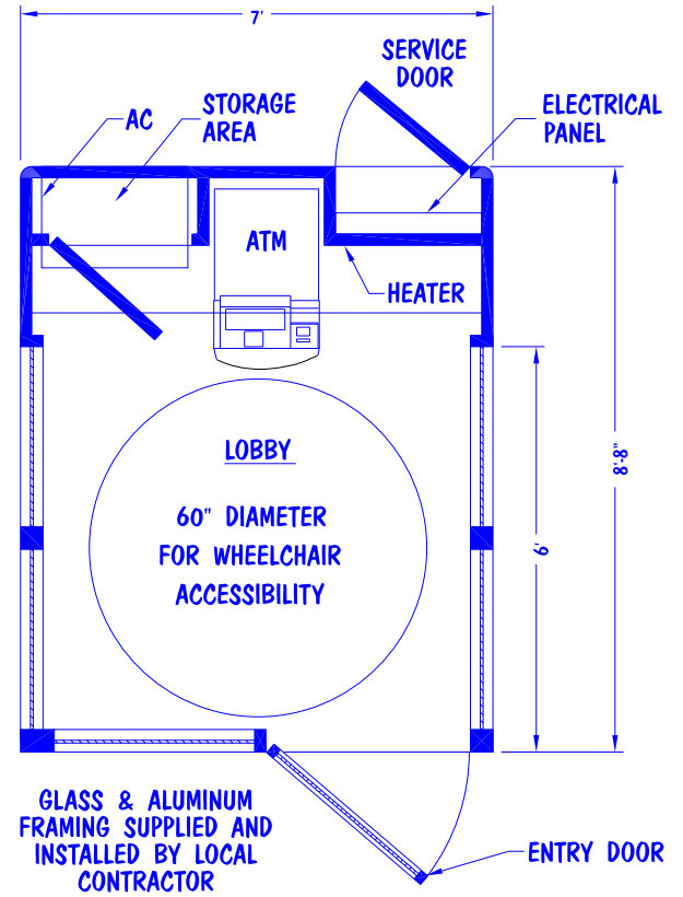
FLOOR PLAN
