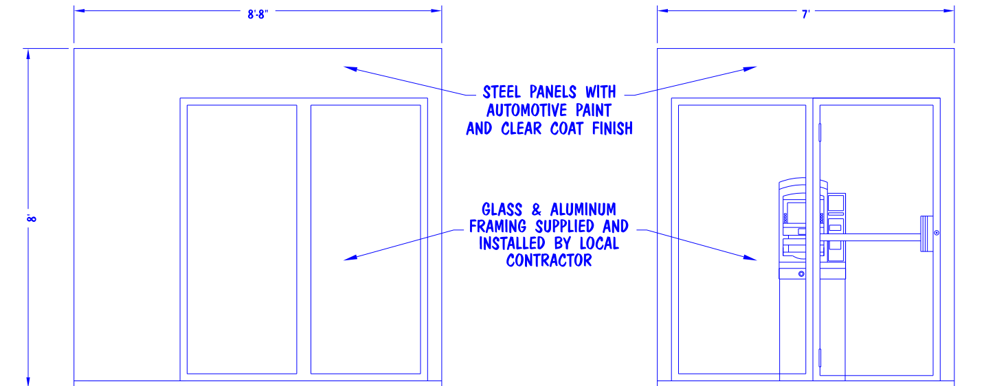
LEFT ELEVATION
