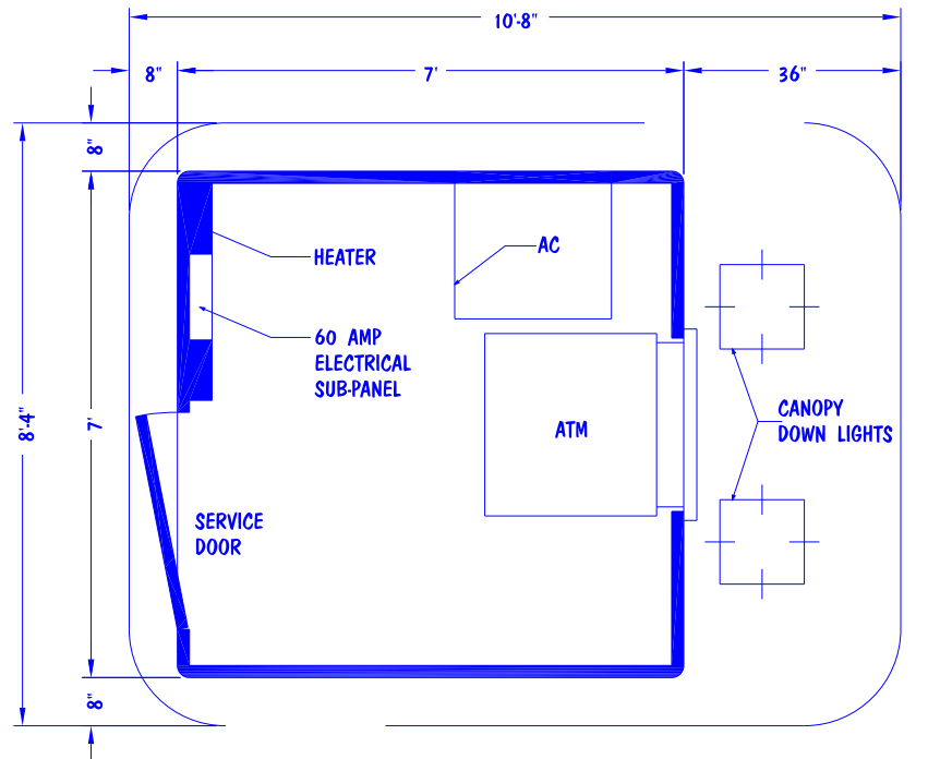
KIOSK #100 WITH OPTIONAL CANOPY FLOOR PLAN
